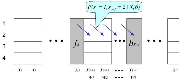
Fig. 3. The contribution of an occurrence of the good string W to A_{12} , computed as the some of the arrow probabilities.
